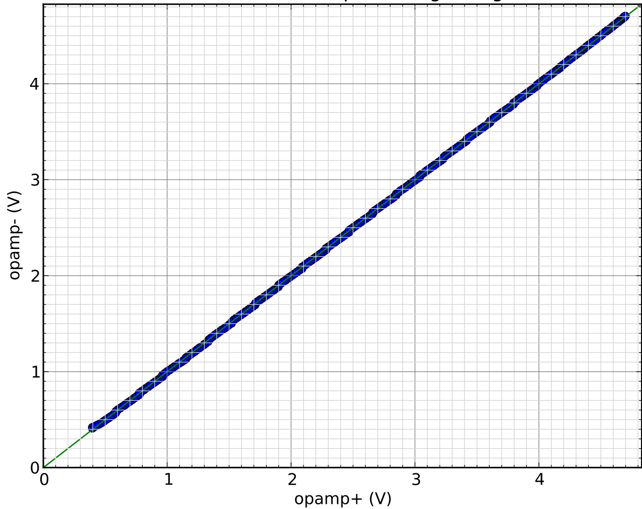
Common-mode input voltage range
