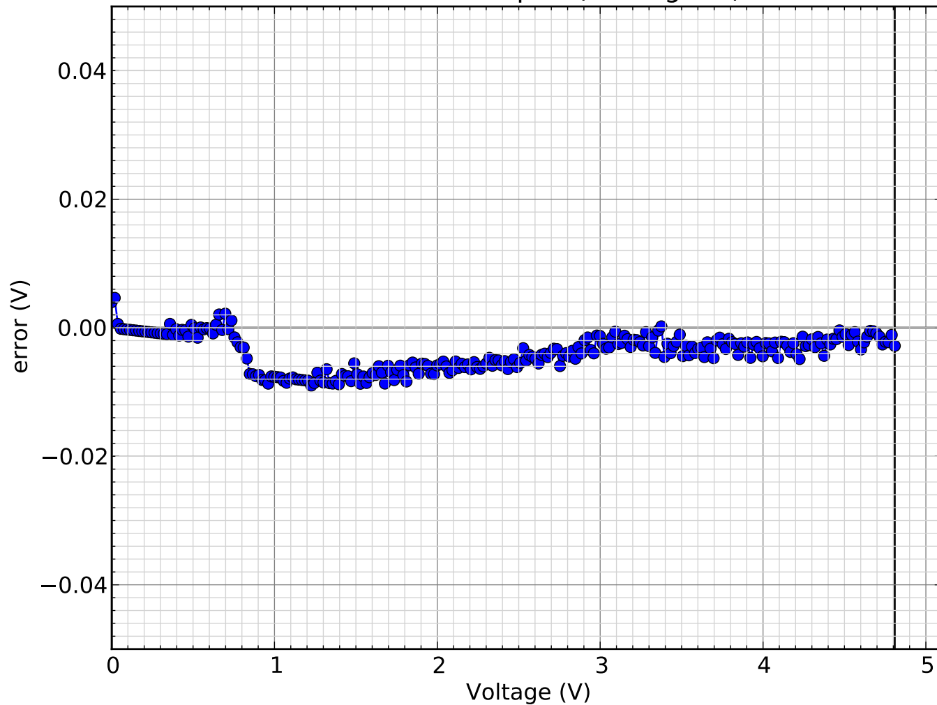
Transfer error plot (ATmega88)
