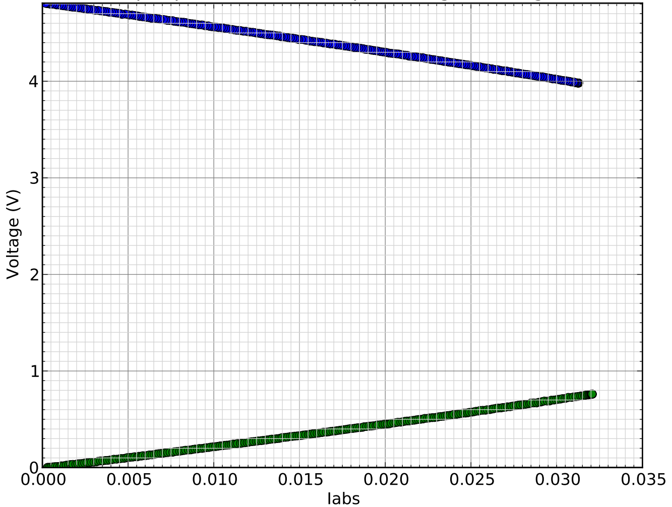
Output pin current vs. output voltage (ATmega88)
