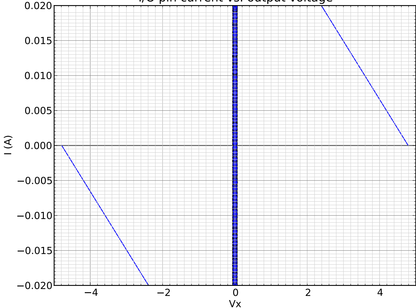
I/O pin current vs. output voltage
