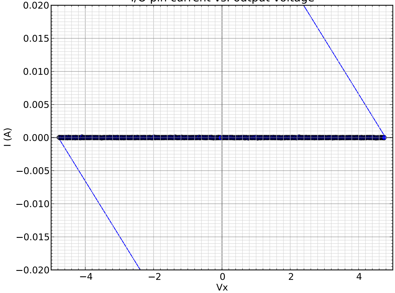
I/O pin current vs. output voltage
